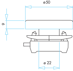
Çiftli Düz Kafalı, Yaylı Double Head With Spring
