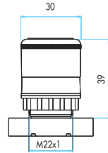
Acil Stop \varnothing 30 mm Emergency Stop \varnothing 30 mm
