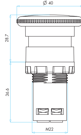
40 mm Mantar Buton 40 mm Mushroom Button
