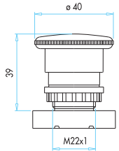
Acil Stop \varnothing 40 mm Emergency Stop \varnothing 40 mm
