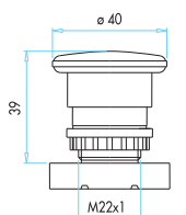
Mantar, Yaylı Mushroom
