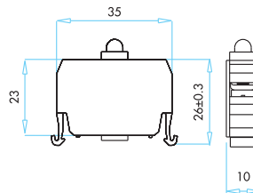
C Serisi Ledli Işıklı Blok-Kutuluk C Series Illumination Block With Led-For Box
