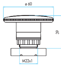
Acil Stop \varnothing 60 mm Emergency Stop \varnothing 60 mm
